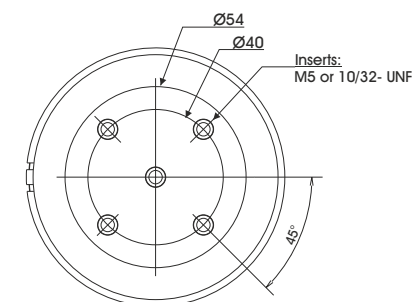
Armature 54
