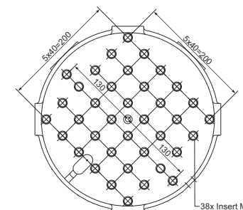
Armatur 300 (Standard)
